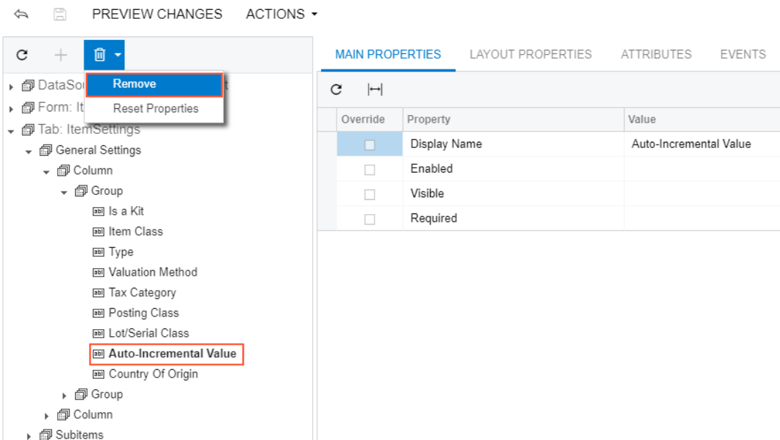
Figure: Removing the selected UI control
