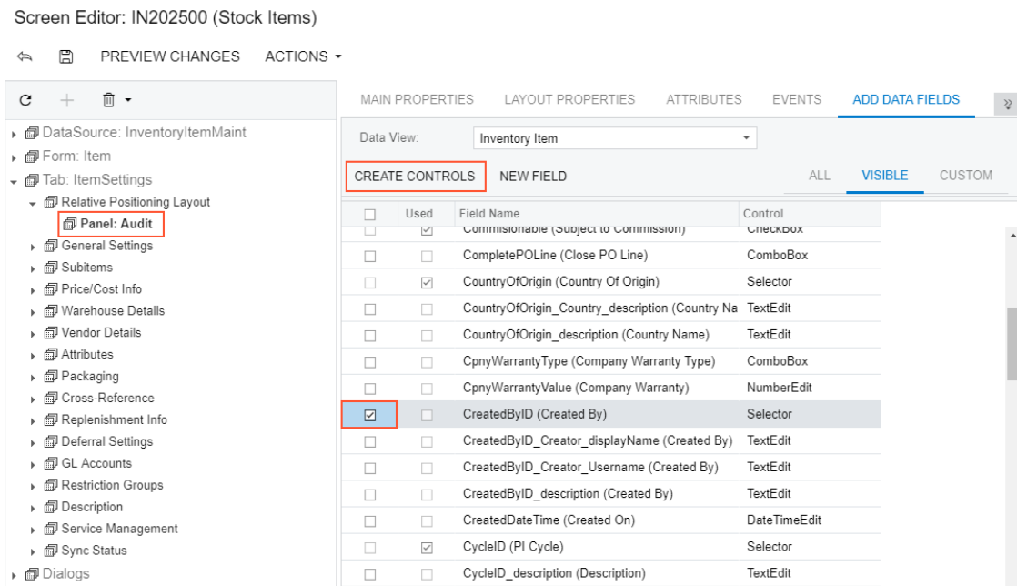
Figure: Adding a UI control to the PXPanel container control
