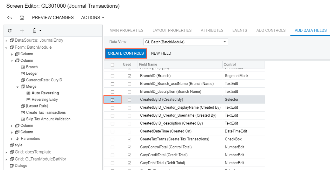
Figure: Creating a control below the selected one in the tree of controls
