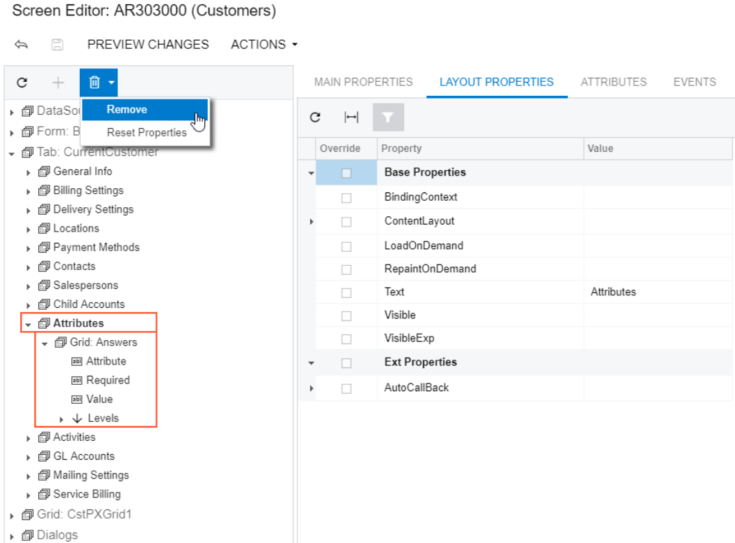
Figure: Deleting a UI element
