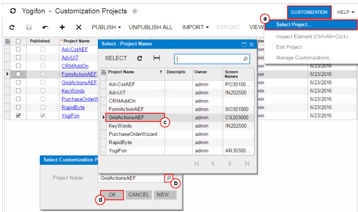
Figure: Selecting a customization project from the Customization menu
