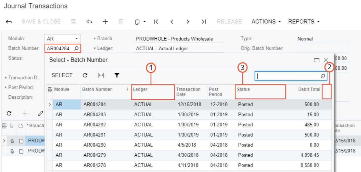
Figure: Viewing the current structure and content of the lookup window
