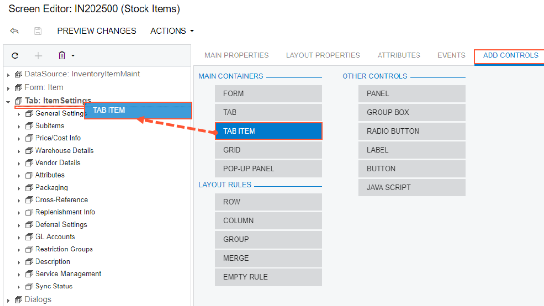
Figure: Adding a tab item to the left position on the tab area of the Stock Items form
