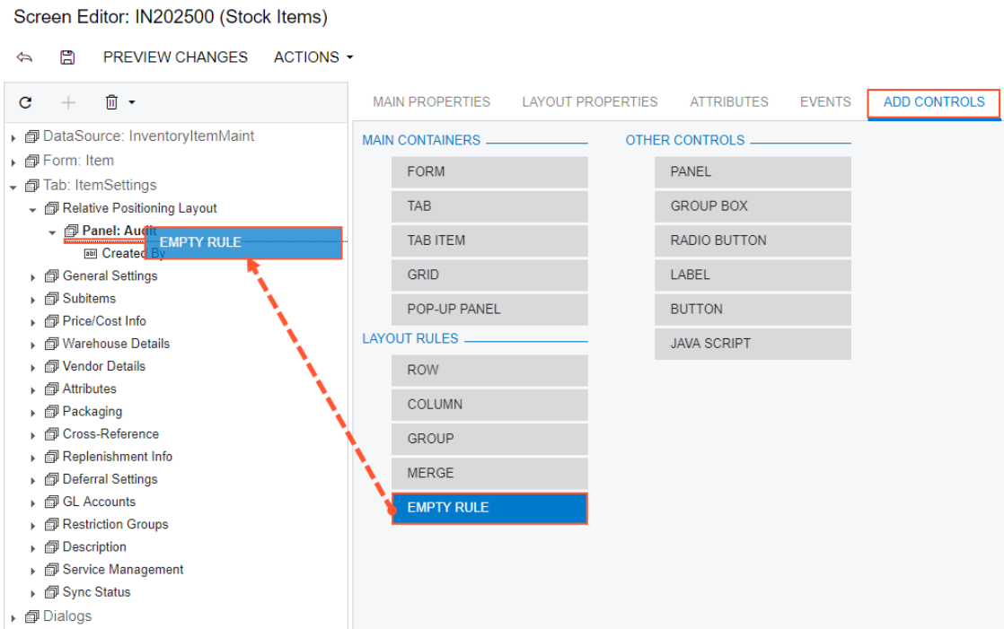
Figure: Adding the PXLLayoutRule onto the panel
