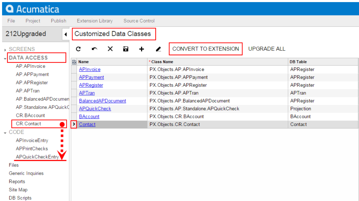
Figure: Converting the DAC item to the Code item
