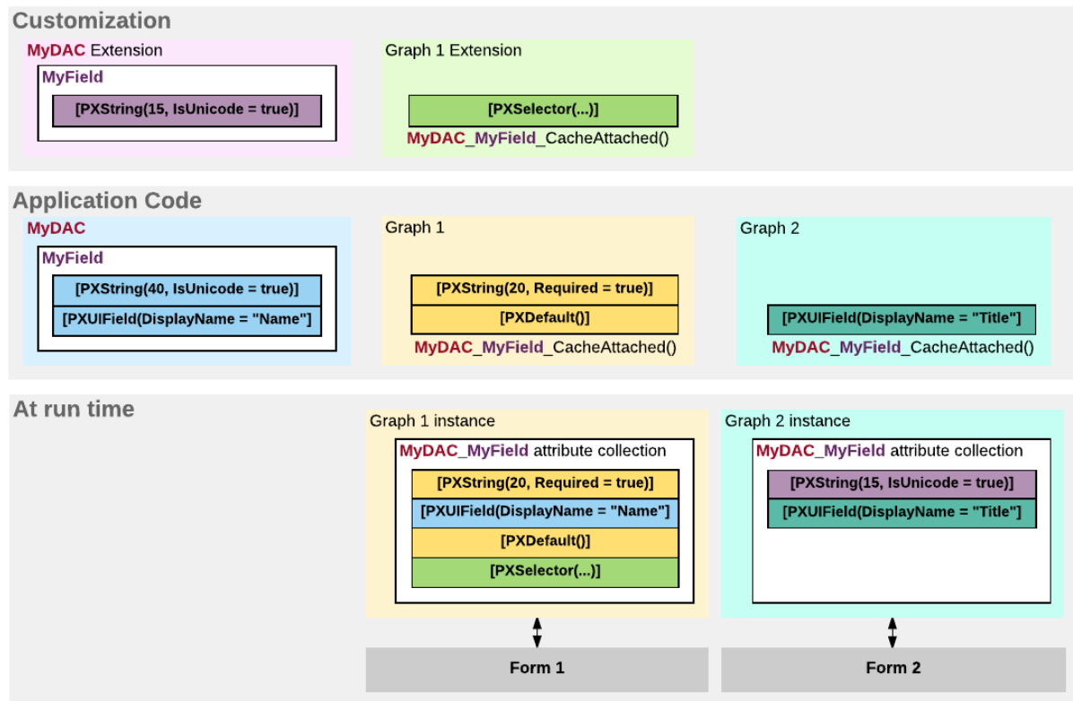
Figure: Example of the customization of attributes for a data field on the DAC and graph levels
